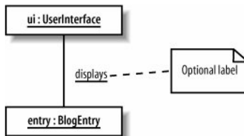
Figure 6-6. To play some tunes, a BlogEntry object is connected to a UserInterface object
