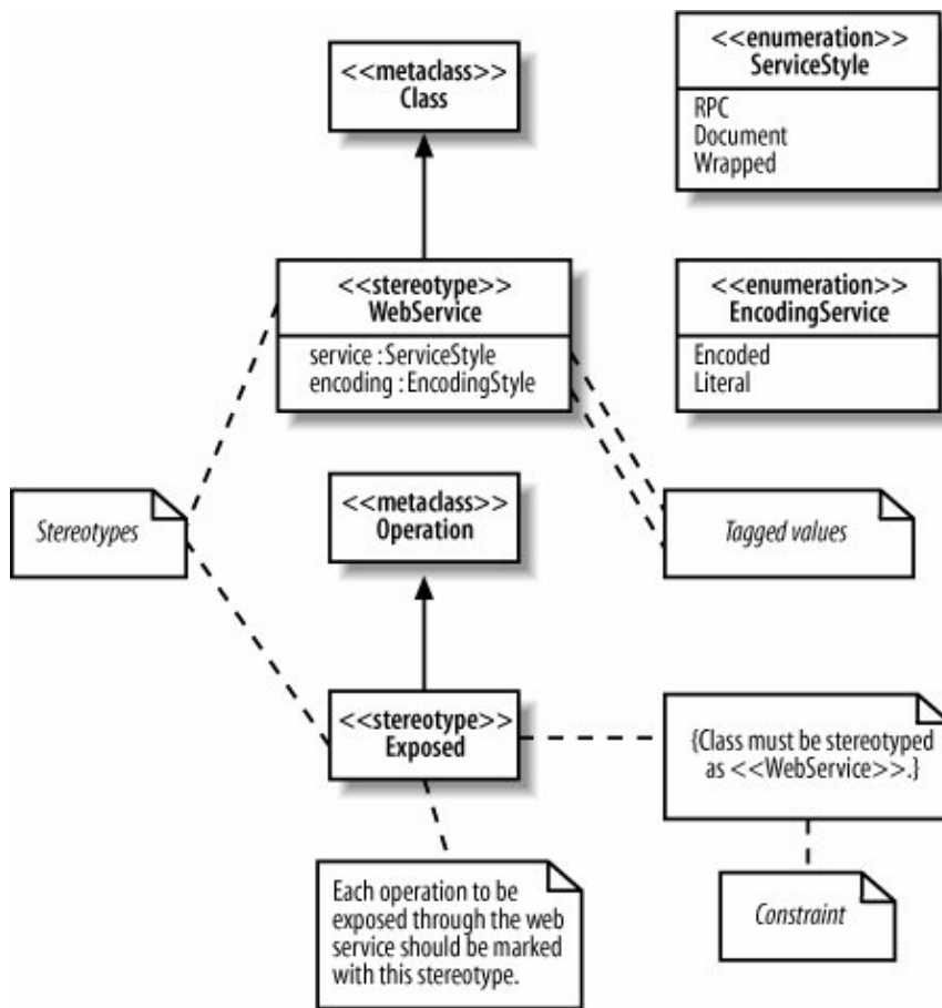
Figure B-6. Creating a new profile that contains two stereotypes, Exposed and WebService , and some associated tagged values and constraints
