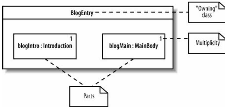
Figure 11-6. The internal structure of the BlogEntry class
