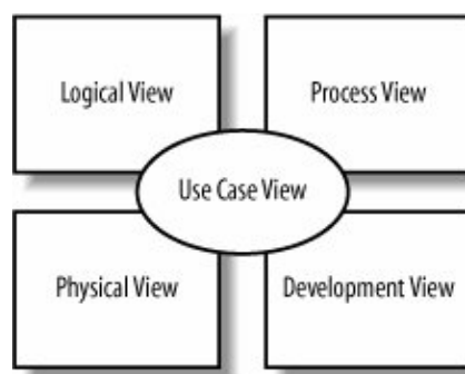
Figure 1-7. Philippe Kruchten's 4+1 view model
