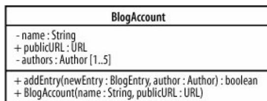
Figure 4-20. The BlogAccount(..) constructor must always return an instance of BlogAccount , so there is no need to explicitly show a return type
