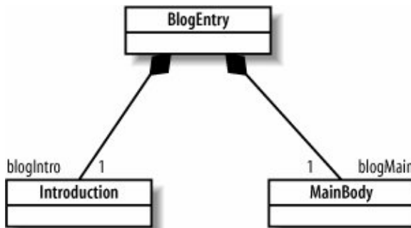
Figure 11-2. Class diagram showing that BlogEntry contains Introduction and MainBody
