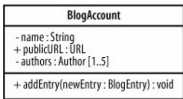
Figure 4-17. Adding a new parameter to the addEntry operation saves a bit of embarrassment when it comes to implementing this class; at least the addEntry operation will now know which entry to add to the blog!
