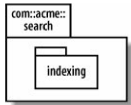
Figure 13-6. Flattening nested packages
