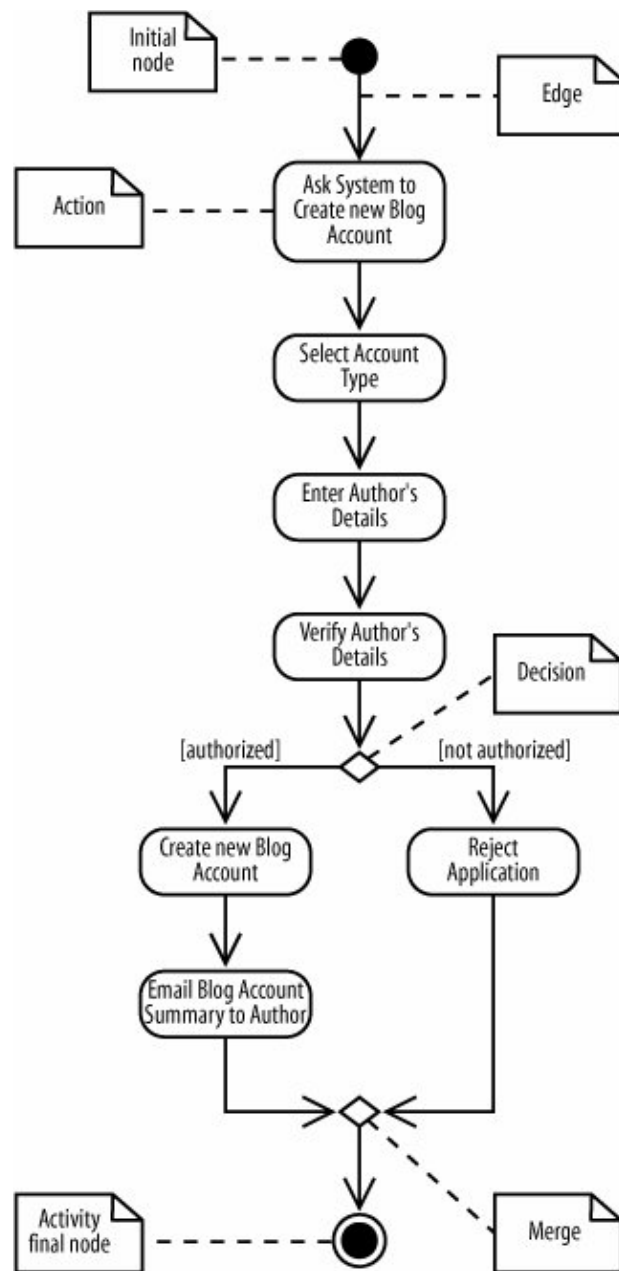
Figure 3-2. Activity diagrams model dynamic behavior with a focus on processes; the basic elements of activity diagrams are shown in this blog account creation process
