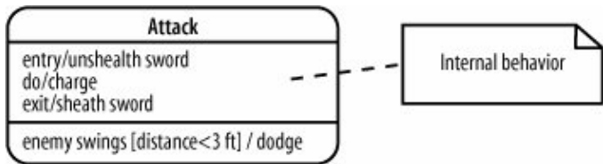
Figure 14-15. The middle compartment shows internal behavior
