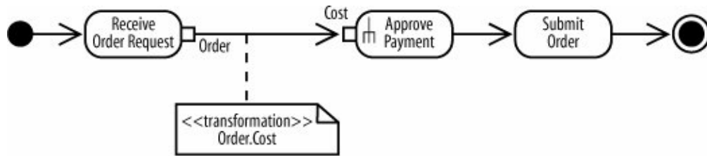
Figure 3-17. Transformations show where input parameters come from
