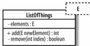
Figure 5-19. A template in UML is shown by providing an extra box with a dashed border to the top right of the regular class box
