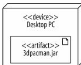
Figure 15-6. The 3dpacman.jar artifact deployed to a Desktop PC node
