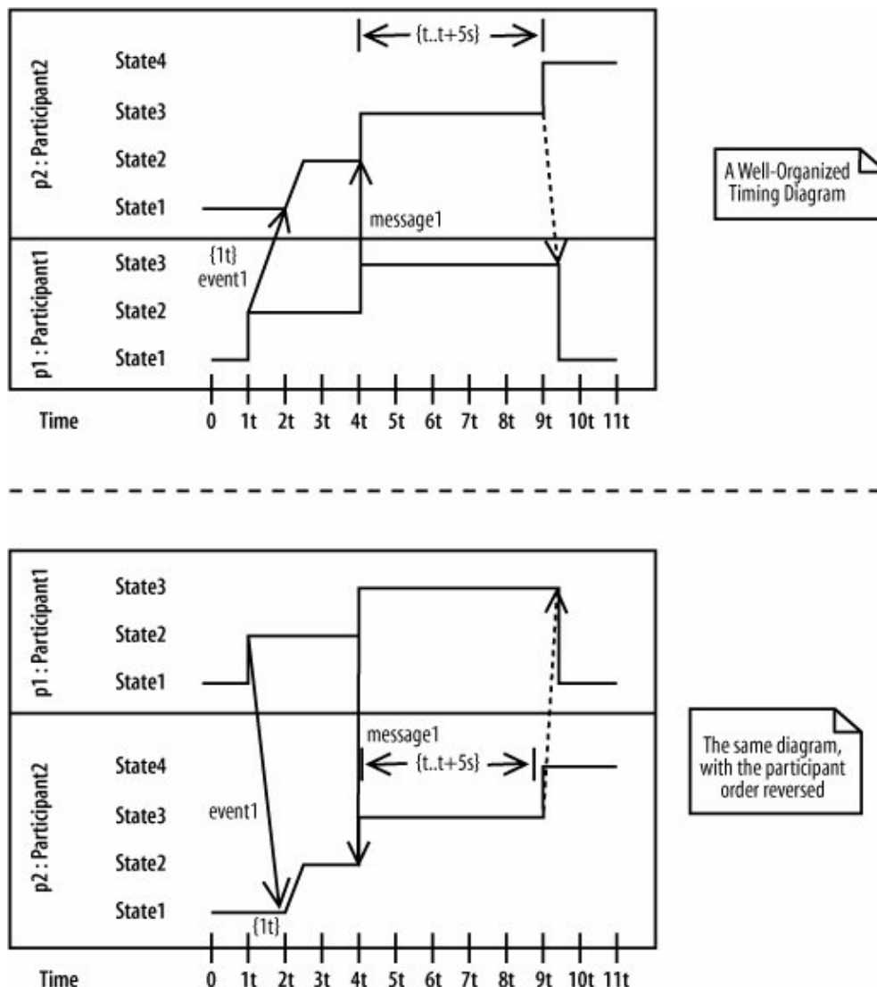
Figure 9-15. The bottom diagram is harder to read, and details are beginning to obscure one another
