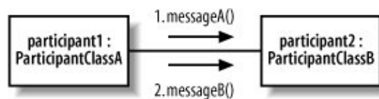
Figure 8-2. Two messages are passed along the link between participant1 and participant2
