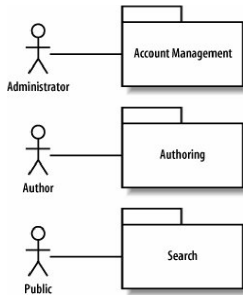
Figure 13-21. Packages enable a higher level view of how actors interact with the system
