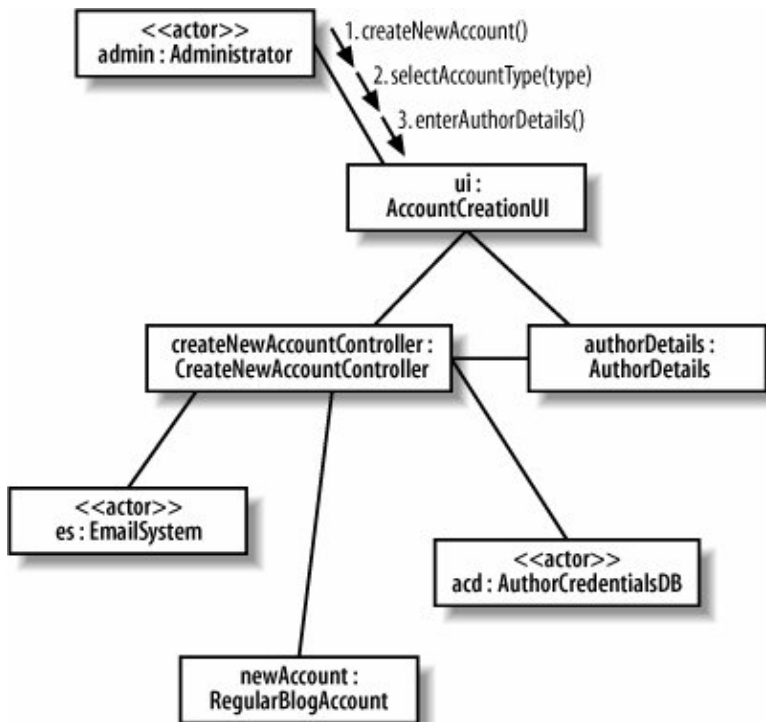
Figure 8-12. The Administrator actor starts things off by passing three separate messages to the ui:AccountCreationUserInterface participant
