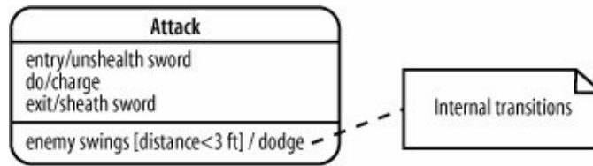
Figure 14-16. The bottom compartment shows internal transitions
