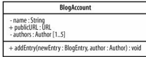
Figure 4-18. As well as passing the new blog entry that is to be added, by adding another parameter, we can also indicate which author wrote the entry
