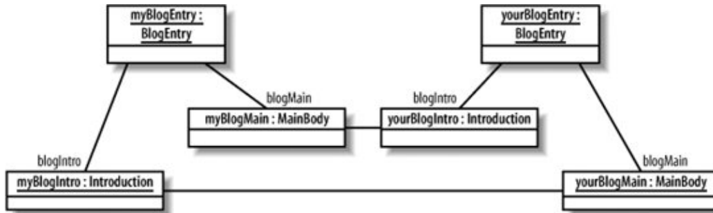
Figure 11-4. Unintended but valid object structure
