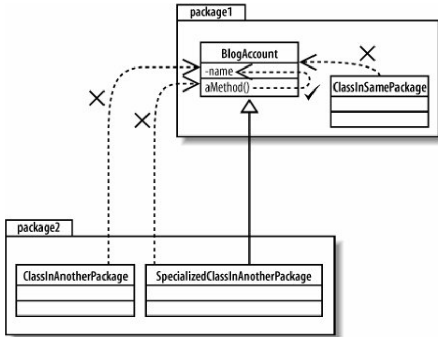
Figure 4-10. aMethod is part of the BlogAccount class, so it can access the private name attribute; no other class's methods can see the name attribute
