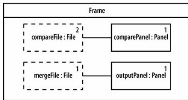
Figure 11-12. A more detailed internal structure diagram that specifies how files and panels relate to each other within a frame
