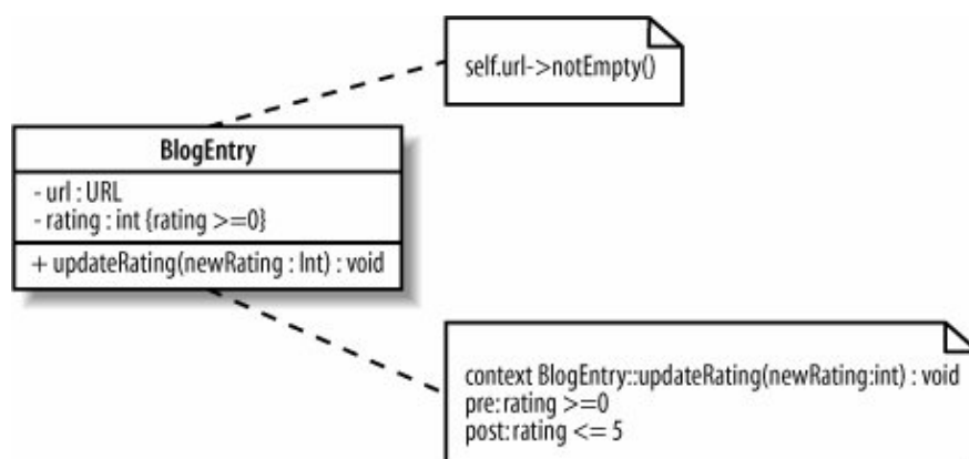
Figure 5-10. Three constraints are set on the BlogEntry class: self.url->notEmpty() and rating >= 0 are both invariants, and there is a postcondition constraint on the updateRating(..) operation
