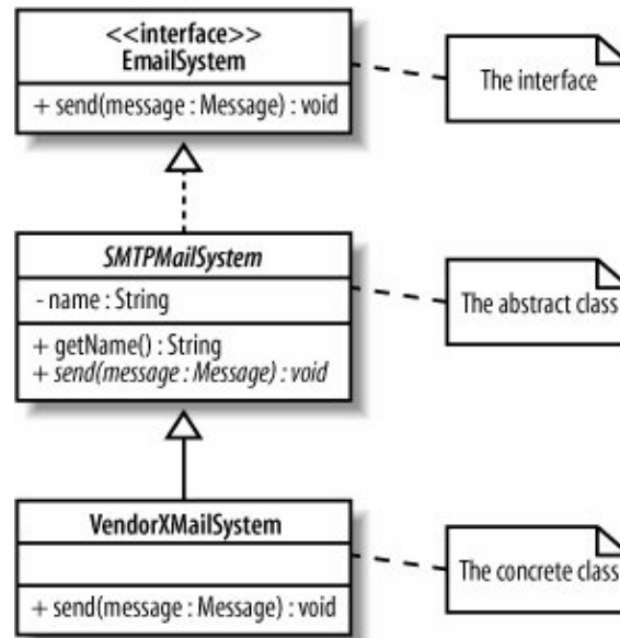
Figure 5-18. Because the SMTPMailSystem class does not implement the send(..) operation as specified by the EmailSystem interface, it needs to be declared abstract; the VendorXMailSystem class completes the picture by implementing all of its operations
