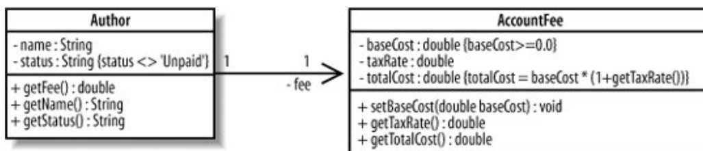
Figure A-2. Example OCL constraints of varying complexity
