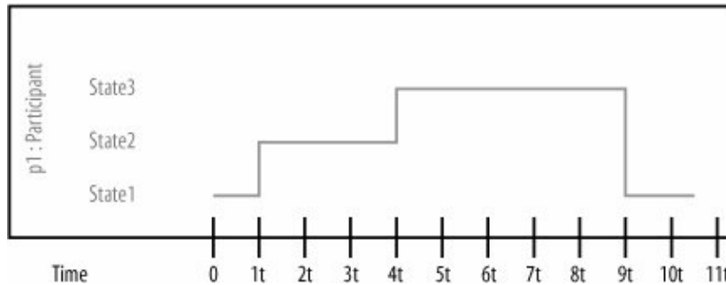
Figure 9-7. Relative time indicators are particularly useful when you have timing considerations such as "ParticipantA will be in State1 for half of the time that ParticipantB is in State2"
