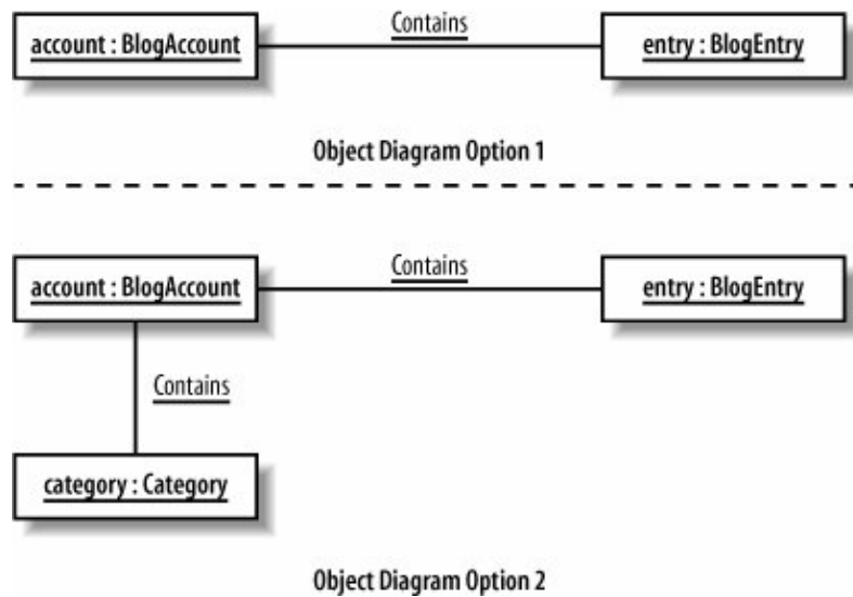
Figure 6-8. A BlogEntry can be associated with a BlogAccount and a set of categories, but there is no rule that states that a BlogEntry must be associated with a category
