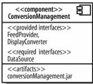
Figure 12-6. Listing required and provided interfaces within the component is the most compact representation
