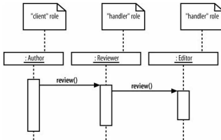
Figure 11-16. Sequence diagram showing how the COR pattern is used in the content approval process
