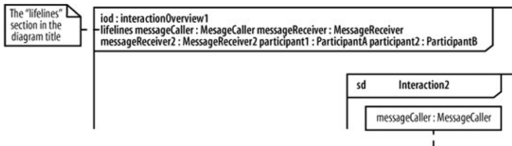
Figure 10-2. The lifelines subtitle shows the combined list of participants involved in the interactions within the overview
