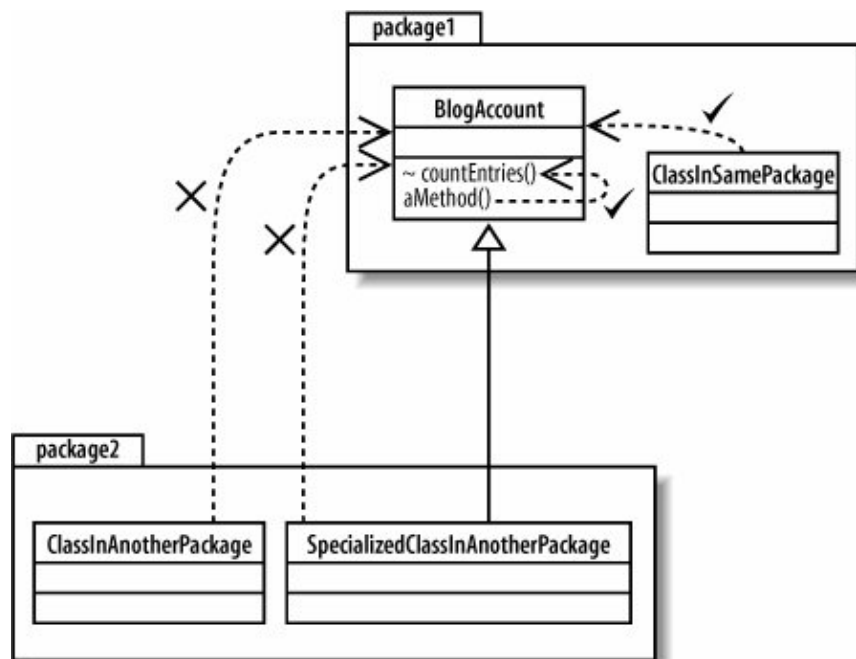
Figure 4-9. The countEntries operation can be called by any class in the same package as the BlogAccount class or by methods within the BlogAccount class itself
