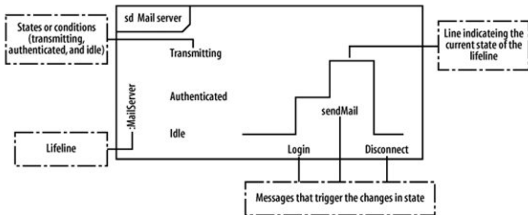
Figure 9-2. Compare this simple yet complete timing diagram for a mail server with the logic analyzer in Figure 9-1
