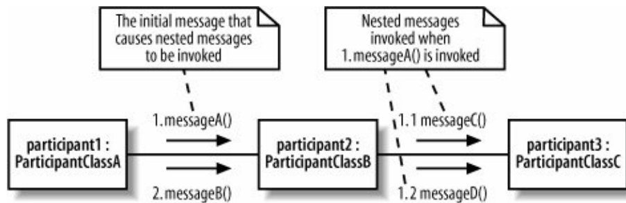
Figure 8-4. messageA() directly leads to nested 1.1 messageC(), followed by nested messageD(), before message 2 is invoked
