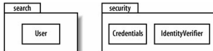
Figure 13-9. Classes in different packages have to provide name scope
