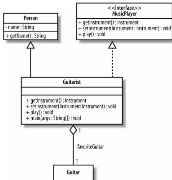
Figure 1-5. Expressing the static structure of the Guitarist class structure in formal UML notation
