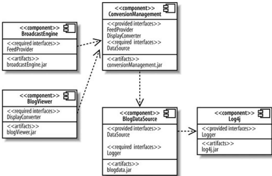
Figure 12-11. Focusing on component dependencies and the manifesting artifacts is useful when you are trying control the configuration or deployment of your system
