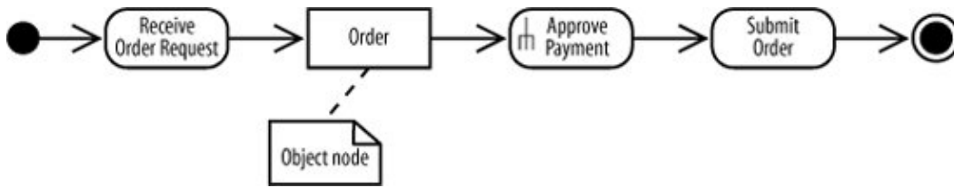
Figure 3-15. The Order object node emphasizes that it is important data in this activity and shows which actions interact with it
