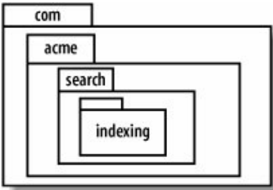
Figure 13-5. Deeply nested packages are common in enterprise applications: the search and indexing packages are shown in a typical package structure for the ACME company
