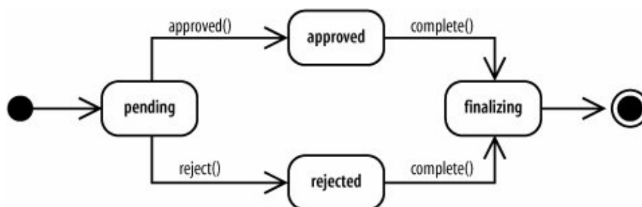
Figure 14-12. The life cycle of an AccountApplication object
