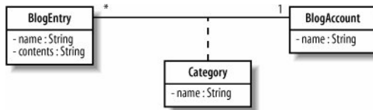
Figure 6-7. When a BlogEntry is added to a BlogAccount, it will be grouped under one or more categories; the Category class is associated with the relationship between a BlogEntry and a BlogAccount
