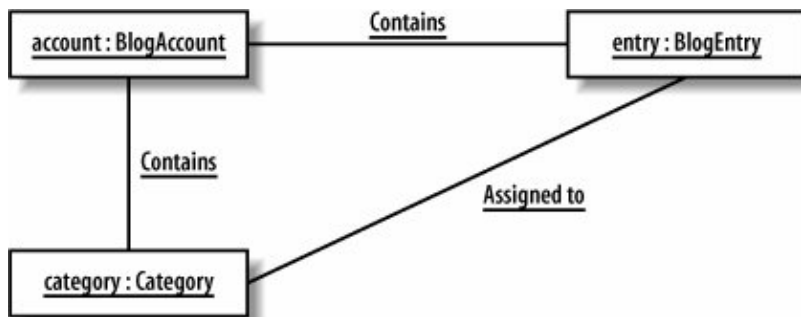
Figure 6-10. The self.category->notEmpty() constraint affects the options available when you create an object diagram, ensuring that an entry is associated with a category for it to be added to a BlogAccount
