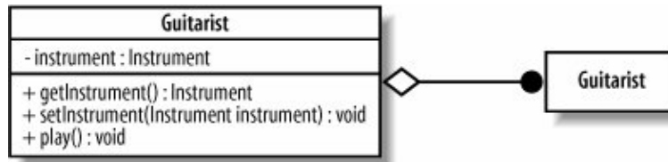
Figure C-3. This diagram is easy to read, even for a novice developer
