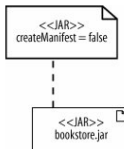
Figure B-4. This tagged value, attached in a note, specifies whether a manifest should be created for the JAR file
