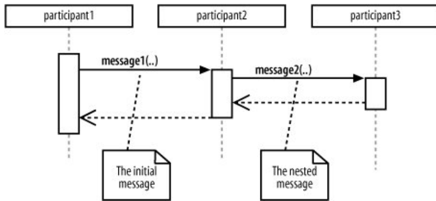
Figure 8-3. Nested messages on sequence diagrams are easy to see; when the initial message, message1(..), is invoked on participant2, participant2 then invokes the nestedmessage2(..) on participant3
