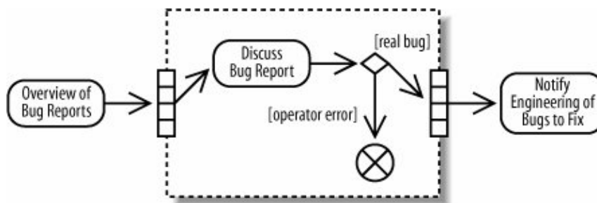
Figure 3-27. The actions in an expansion region are performed for each item in a collection
