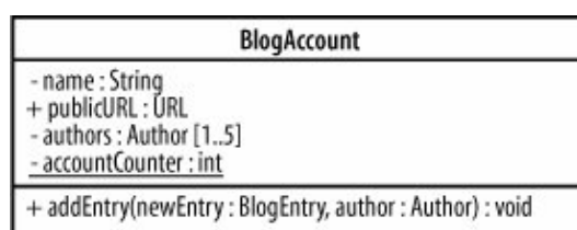
Figure 4-23. An attribute or operation is made static in UML by underlining it; the accountCounter attribute will be used to keep a running count of the number of objects created from the BlogAccount class
