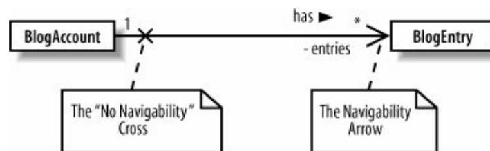
Figure 5-4. If we change Figure 5-3 to incorporate the navigability arrow, then we can declare that you should be able to navigate from the blog to its entries
