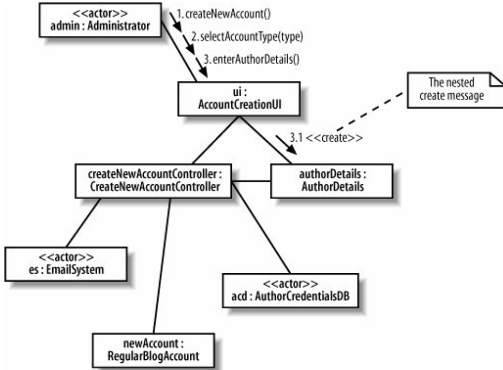
Figure 8-13. When the <<create>> message is added to the communication diagram, its message order number is set to 3.1. to show that it is nested inside the 3. enterAuthorDetails( ) message
