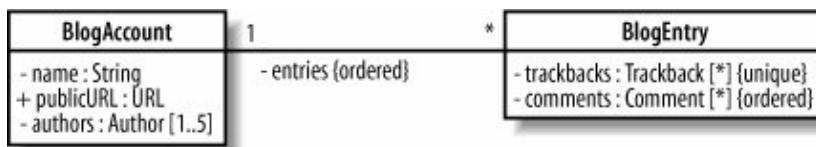
Figure 4-12. Applying several flavors of attribute multiplicity to the attributes of the BlogAccount and BlogEntry classes
