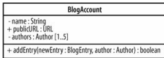
Figure 4-19. The addEntry(..) operation now returns a Boolean indicating whether the entry was successfully added
