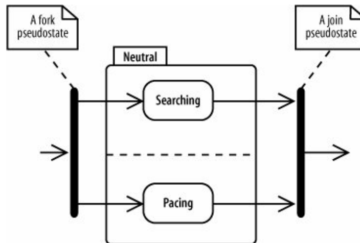
Figure 14-20. Forks and joins show concurrent states
