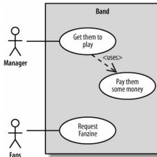
Figure C-2. The OOSE use case notation describes three use cases within a system and the two outside influences/actors that interact with those use cases
