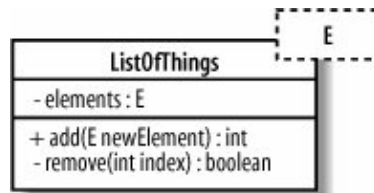
Figure 6-11. The ListOfThings collection can store and remove any class of object to which the E parameter is bound
