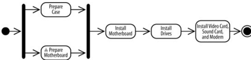
Figure 3-13. Rather than cluttering up the top-level diagram with details of the Prepare Motherboard action, details are provided in another activity diagram
