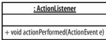
Figure 6-4. The class of this object is ActionListener, but the name or identity is not specified; this object also shows the single actionPerformed(...) method that is required by the ActionListener interface
